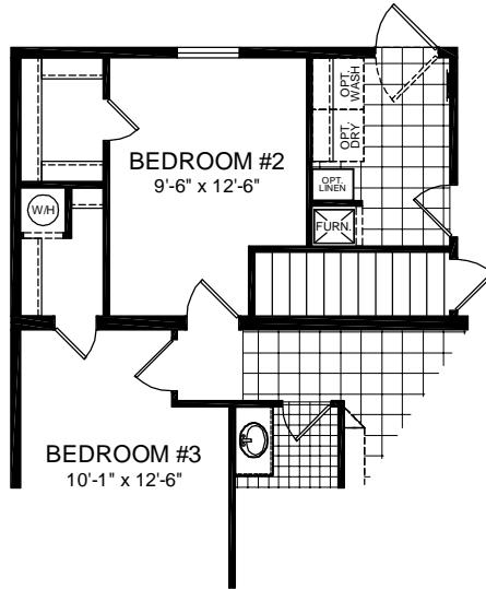
OPT. STAIRWELL
