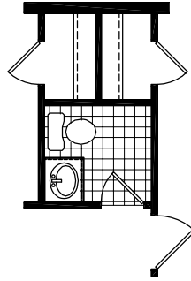
OPT. HALF BATH
