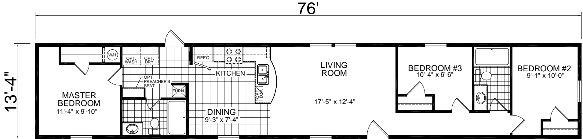
MODEL 108 3 BEDROOM, 2 BATH TOTAL AREA: 1013 SQ. FT.
