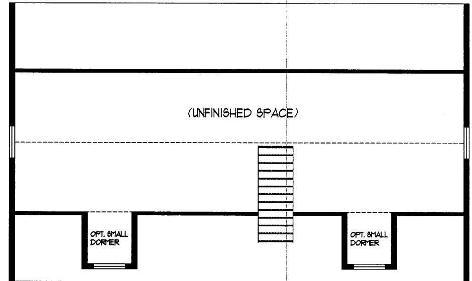
OPT. SECOND FLOOR
