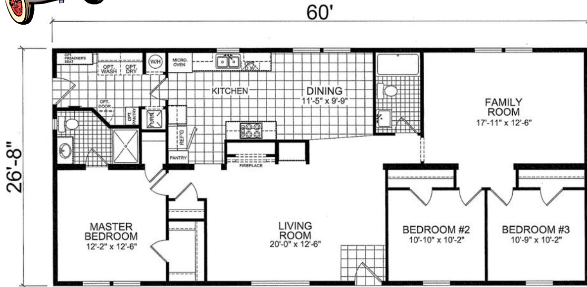
MODEL 933 3 BEDROOM, 2 BATH ACTUAL SIZE: 26'-8" x 60'-0" TOTAL AREA: 1600 SQ. FT.
