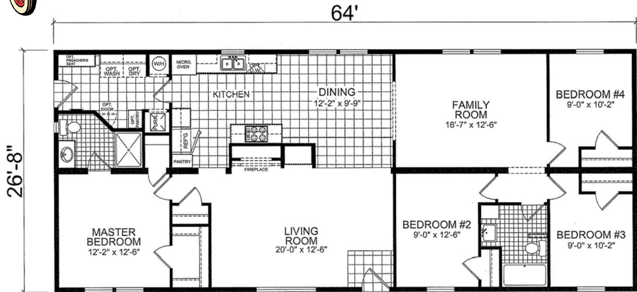
MODEL 934 4 BEDROOM, 2 BATH ACTUAL SIZE: 26'-8" x 64'-0" TOTAL AREA: 1706 SQ. FT.
